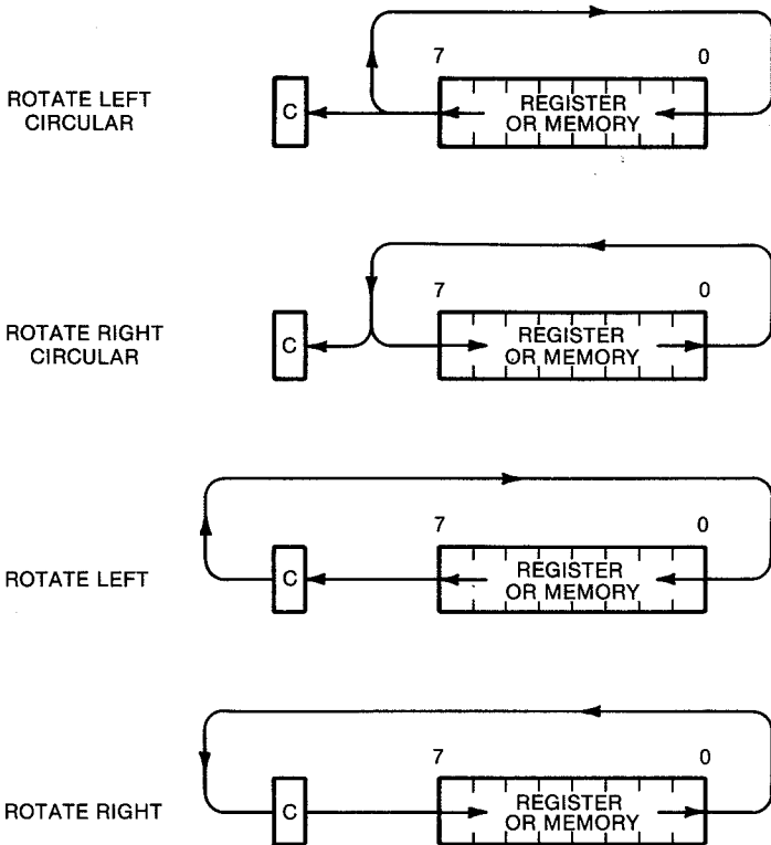
Fig. 12-2. The ROTATE operations.
